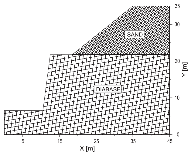
Fig. 5. Cross-section for the numerical simulation of the landslide movement
