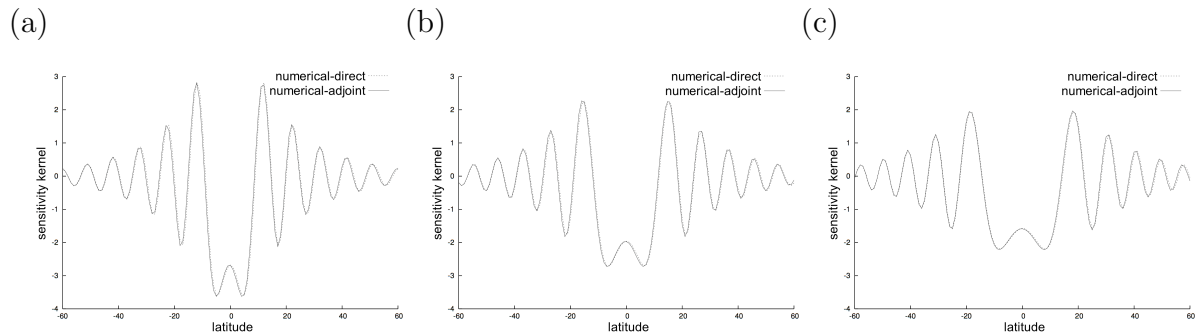
Figure 2.6: Cross-sections of sensitivity kernels for Love waves at 150 s calculated via the “direct” approach (dashed lines) and adjoint method (solid lines), with source at (0°N, 0°E) and receiver at (0°N, 90°E). Sensitivity values are plotted as a function of latitude only, along three chosen meridians, namely (a) 10°, (b) 20° and (c) 45°.
