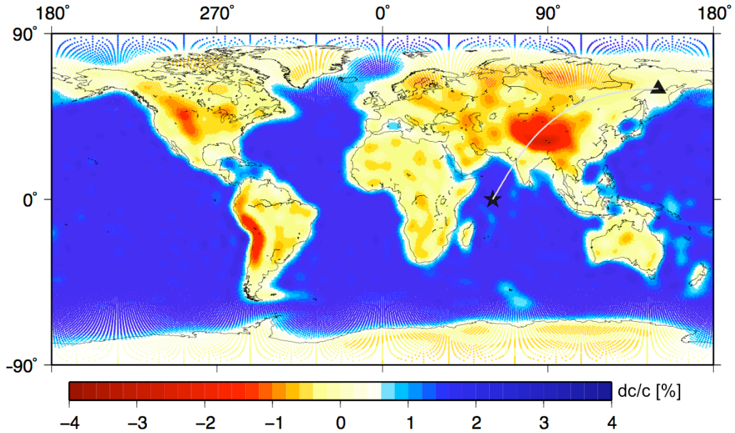
Figure 2.9: 150 s Love-wave phase-velocity map based on Crust-2.0 (Bassin et al. 2000) and an isotropic upper-mantle model. The phase-velocity heterogeneities are represented by a spherical harmonic expansion with degrees l \leq 40 , resulting in a low-pass filtered phase-velocity map (the membrane analogue has physical meaning in a smooth Earth regime). Phase-velocity values are projected onto our hexagonal grid, and plotted as colored dots at the centre of each of its cells (122,882 total cells). Source and receiver are denoted by the star and triangle connected by the source-receiver great circle, which crosses the Tibet anomaly. Phase-velocity anomalies are given in percent with respect to PREM.
