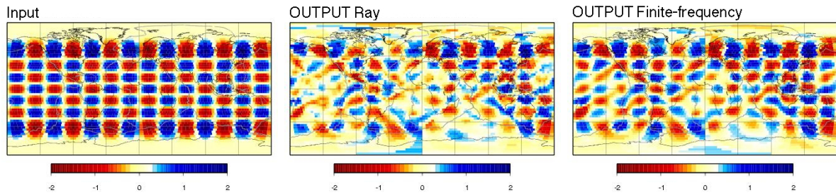
Figure 3.10: Using statistical noise in the synthetic dataset, solutions for Love waves at 150 s period and an input model of 2% perturbations are shown: (a) with a checkerboard with l = 13 and m = 7 and (b) with a checkerboard with l = 20 and m = 10 . The input models are shown in the left column, solutions of the ray-theoretical inversions in the middle and finite-frequency inversions on the right column.
