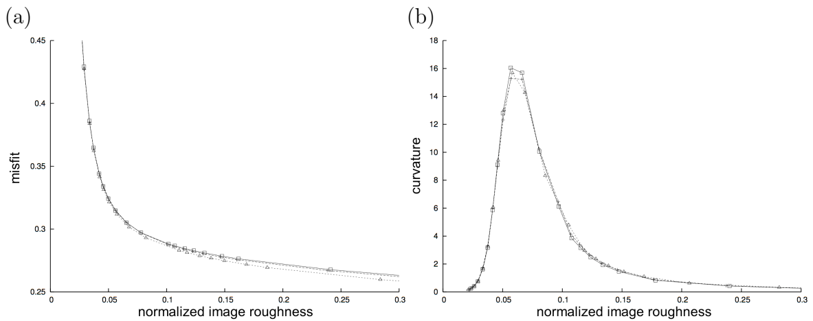
Figure 2.13: Trade-off analysis for the phase-velocity inversions of section 2.4.4 (homogeneous starting model). (a) L-curves for solutions derived from ray theory (dotted line, triangles), analytical Born theory (dashed line, pluses), and numerical-adjoint kernels (solid line, squares). (b) Curvature of the curves shown in (a). Image roughness is defined and normalized as in Boschi (2006).
