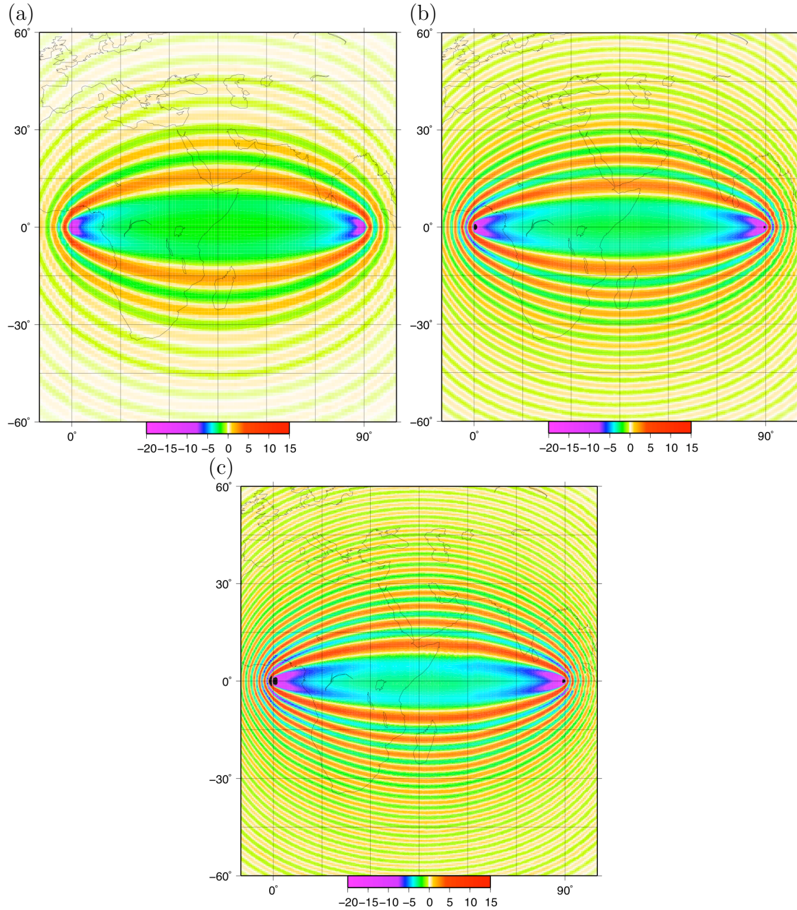
Figure 2.8: Numerical-adjoint kernels for Love waves at (a) 150 s, (b) 100 s and (c) 75 s periods, in a homogeneous starting model. The source is located at (0^\circ\text{N}, 0^\circ\text{E}) , the receiver at (0^\circ\text{N}, 90^\circ\text{E}) .
