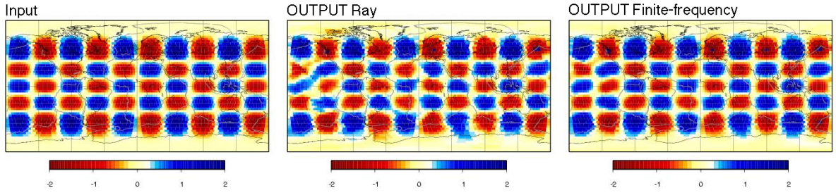
Figure 3.8: Inversions for Love waves at 150 s period and input models of 2% perturbations and different scalelengths of heterogeneities: (a) checkerboard defined as a single spherical harmonic of degree l = 9 and order m = 5 , (b) checkerboard with l = 13 and m = 7 and (c) checkerboard with l = 20 and m = 10 . The input models are shown in the left column, solutions of the ray-theoretical inversions in the middle and finite-frequency inversions on the right column.
