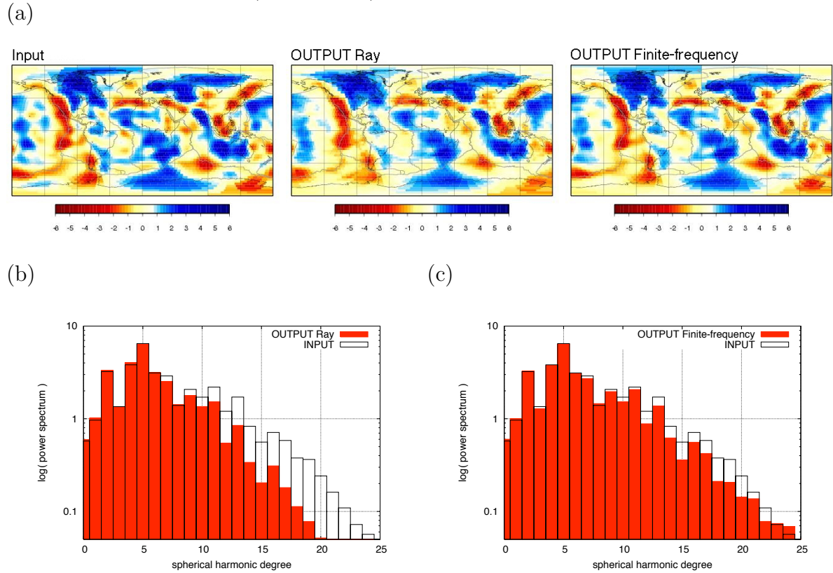
Figure 3.12: Realistic input model TW96 solved for Love waves at 150 s period. (a) The input model is shown on the left, the ray-theoretical inversion in the middle and the finite-frequency inversion solution on the right. The corresponding power spectrum up to spherical harmonic degree 25 of (b) the ray-theoretical solution image (red bars) and (c) the finite-frequency solution image (red bars) are plotted against the initial power spectrum of the input model (black boxes).
