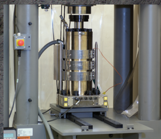
Model 816 Rock Mechanics Test System
