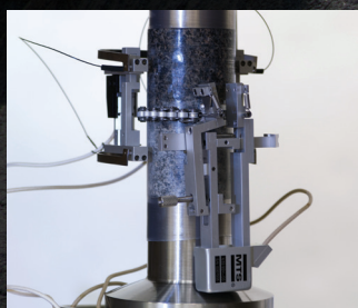
MTS 632 series In vessel Extensometers
