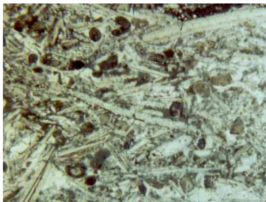
A: Biograinstone microfacies. Sample AR 5 from the Sundance Formation at section Alcova Reservoir (scale is 1,1 cm for the long side of the photo). The particles (pelecypods and crinoids) are poorly sorted and densely packed. The sample has a strong rudstone-like texture.
