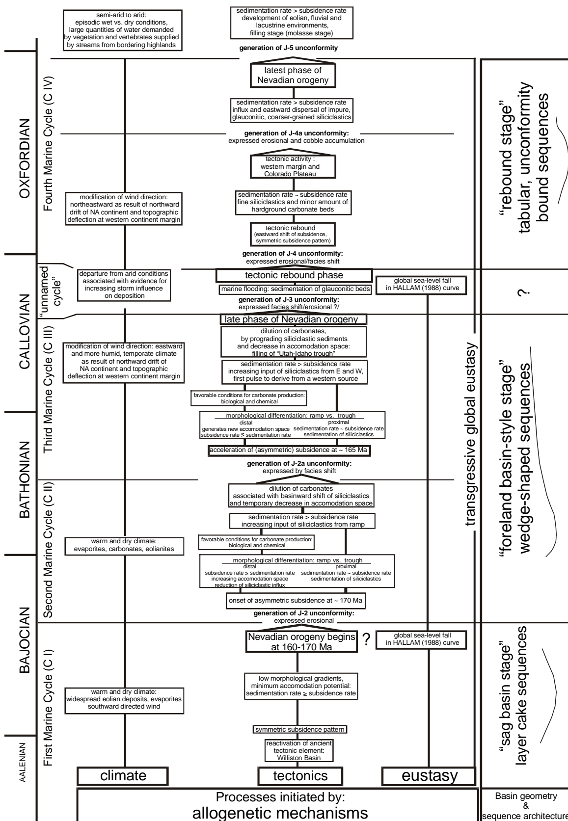
Figure 11-3: Process flow diagram to display the interplay between the allogenetic factors climate, tectonism and eustasy on facies evolution and sequence architecture.
