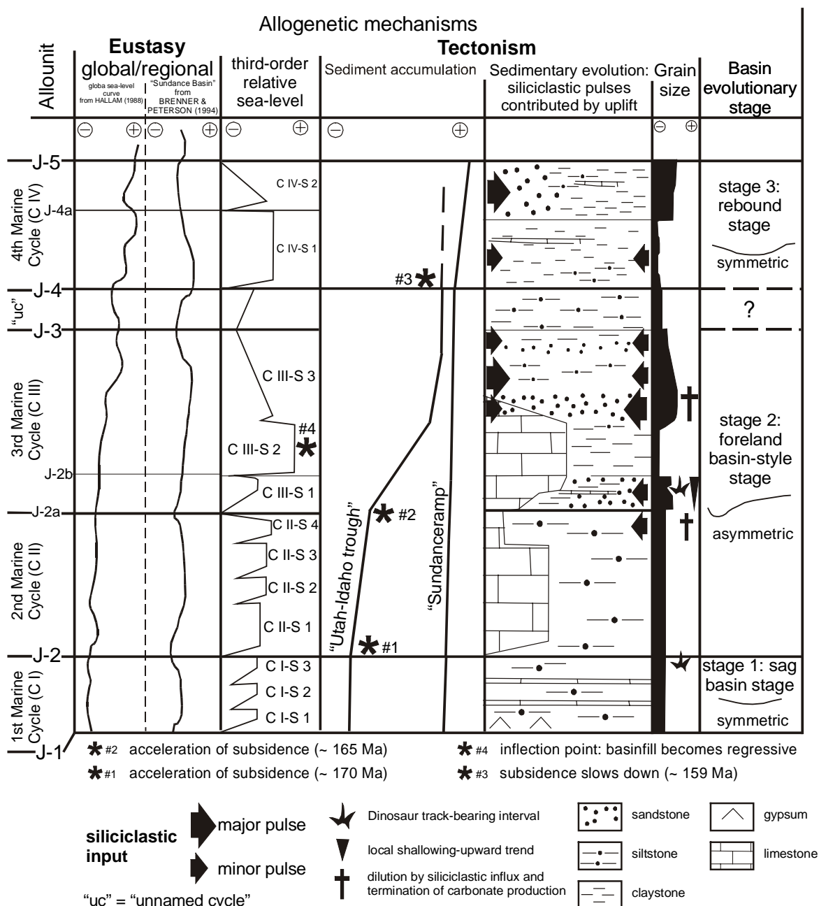
Figure 11-2: Diagram to display the interplay and timing of allogenetic influences on deposition in the “Sundance Basin”.
