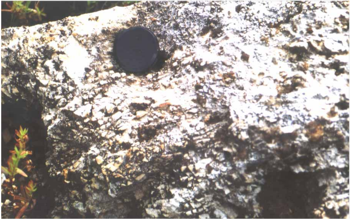
Figure 3-26: Honeycombed, well-sorted collapse breccia in the Gypsum Spring Member of the Twin Creek Limestone at section Poker Flat section (PF). Lense cap is 6 cm in diameter.
