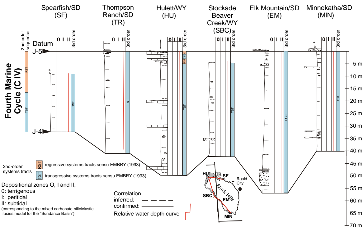
Figure 7-14: Sequence and cyclostratigraphic correlation of the Fourth Marine Cycle (C IV) in the Black Hills. For explanation of lithologic signatures see Figure 7-9.
