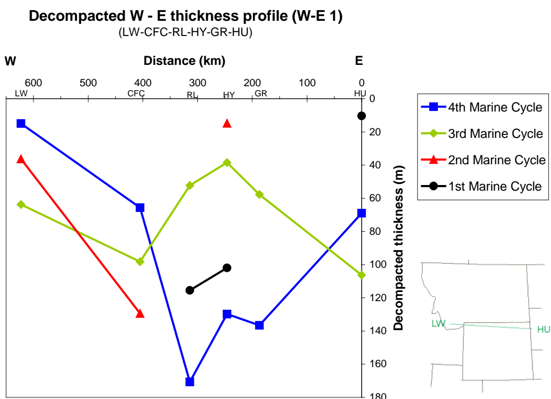
Figure 9-4: Decompacted west-east oriented thickness profiles for the sedimentary cycles C I, C II, C III, C IV trending from section Hulett (HU) to section Little Water Creek (LW).
