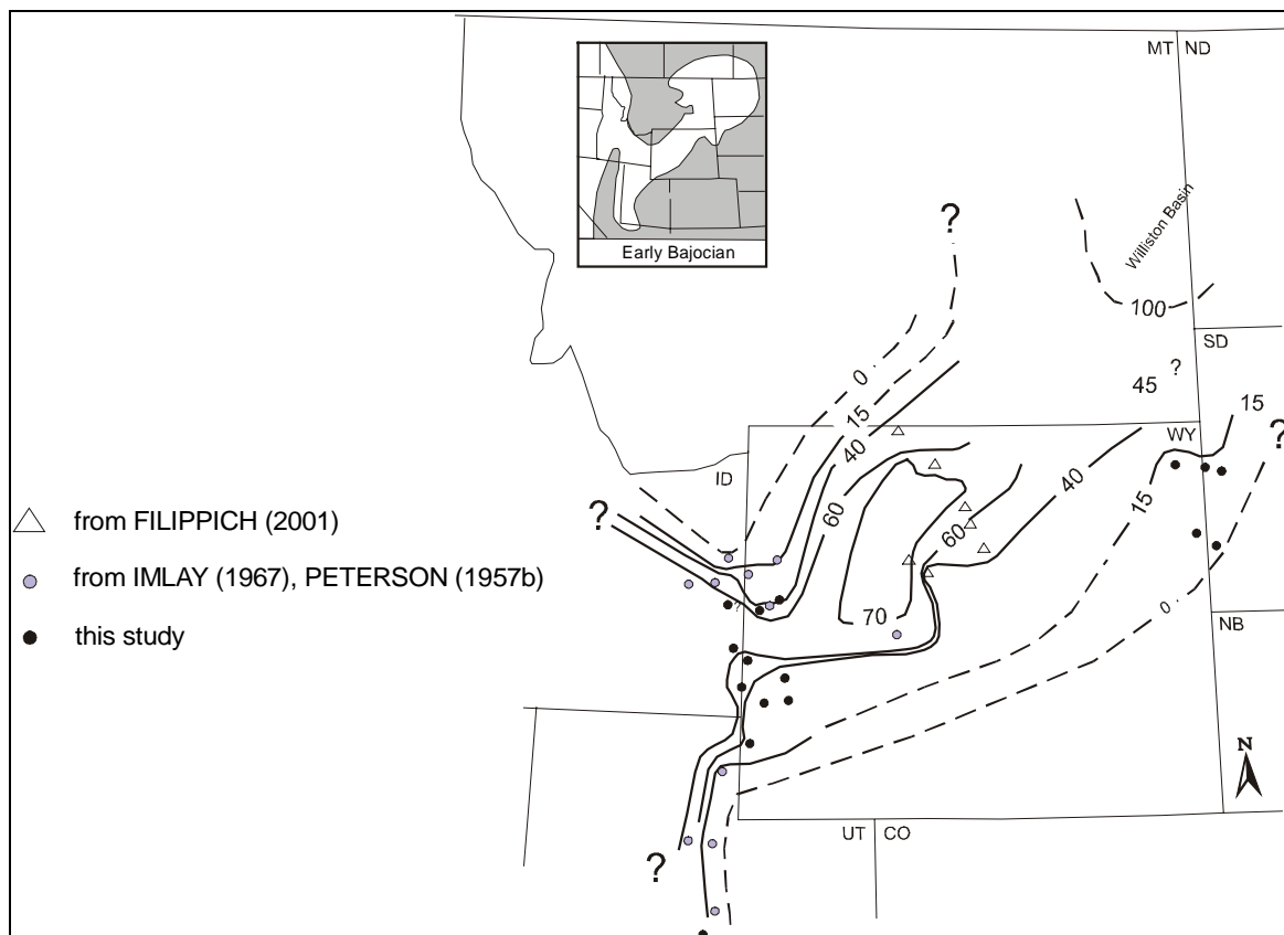
Figure 7-2: Isopach map for compacted stratal thickness of the First Marine Cycle (C I).
