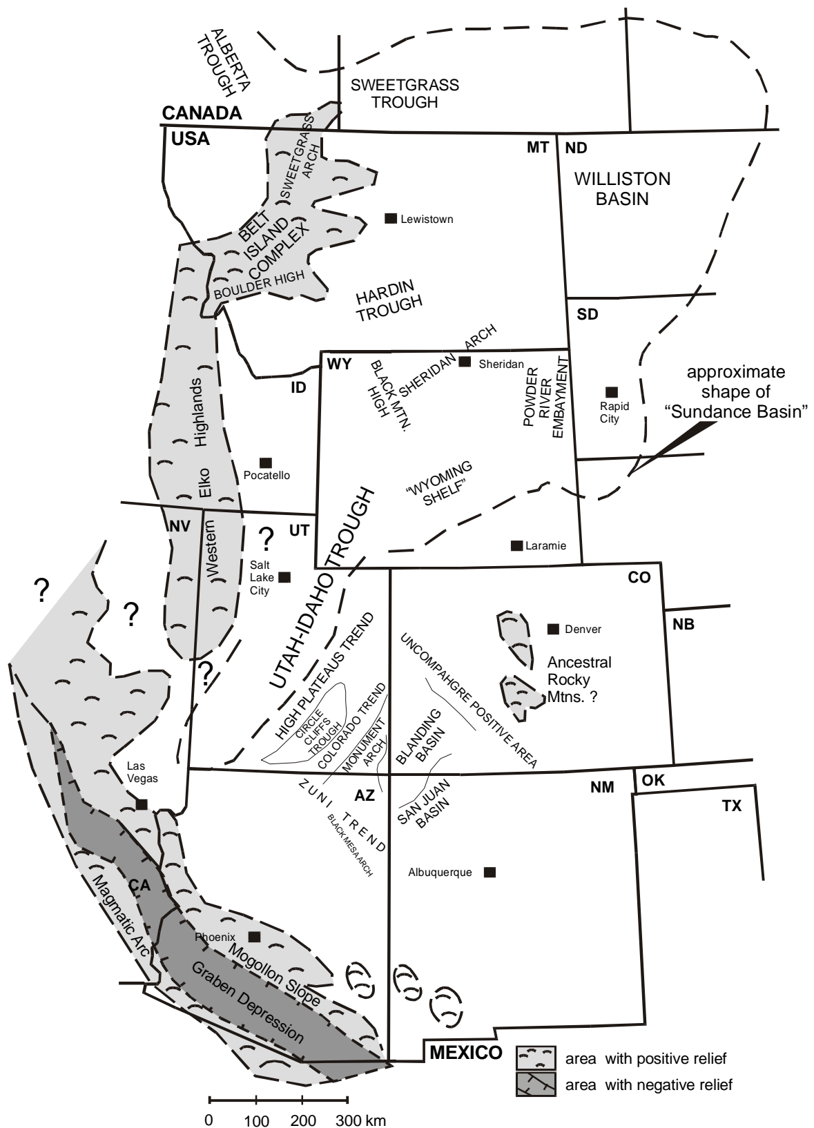
Figure 2-2: Paleogeographic map of the "Sundance Basin" structure with individual paleotectonic elements for the Middle and Late Jurassic. Compiled from PETERSON (1954; 1957a and b; 1958), KOCUREK & DOTT (1983), BLAKEY et al. (1983), BLAKEY (1988), PETERSON, F. (1986; 1994), BRENNER (1983), IMLAY (1980), SCHMUDE (2000).
