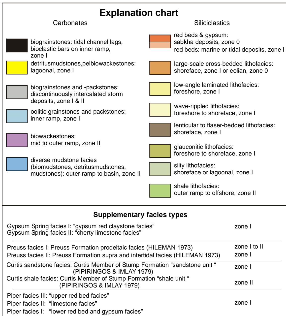
Figure 5-1: Explanation chart for color code of facies types.
