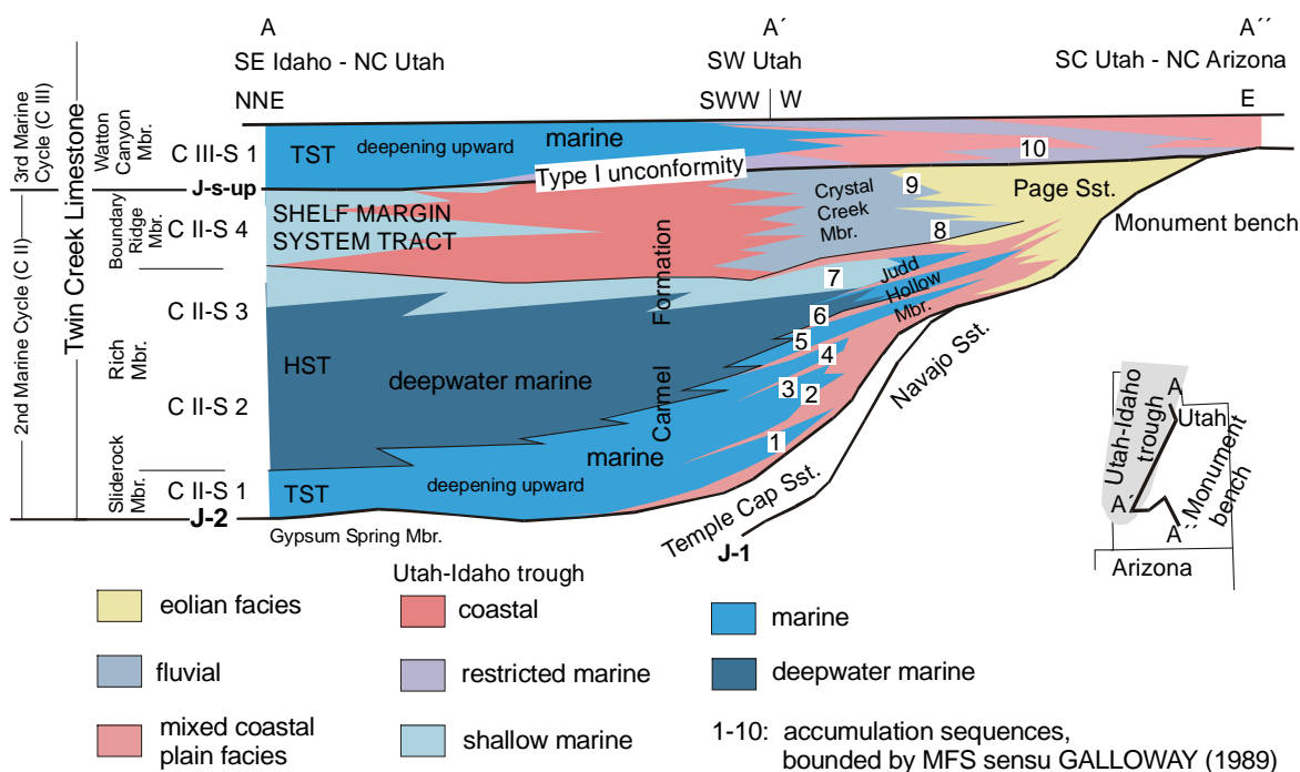
Figure 8-3: Regional genetic sequence stratigraphy sensu GALLOWAY (1989), stratigraphy and facies distribution of Bajocian and Bathonian rocks in the southern parts of the “Sundance Basin”, modified from BLAKEY et al. (1996). C II and C III and subordinate sequences are added from investigations in this work.
