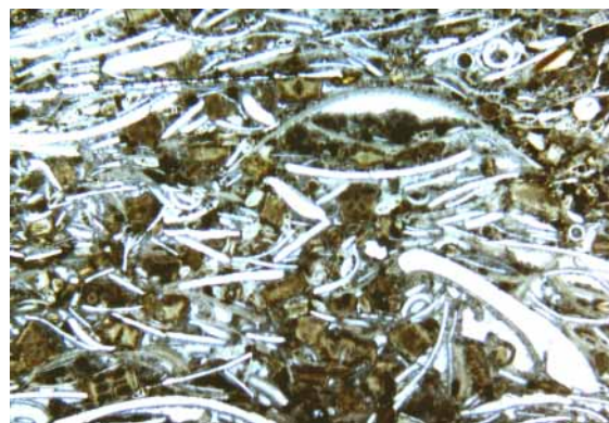
D: Biopackstone microfacies. Sample MIN 10 from the Sundance Formation at section Minnekatha (scale is 1,1 cm for the long side of the photo). The sample shows a strong affinity to a rudstone texture. The particle spectrum comprises crinoidal columns and pelecypod shells with micritic envelopes.
