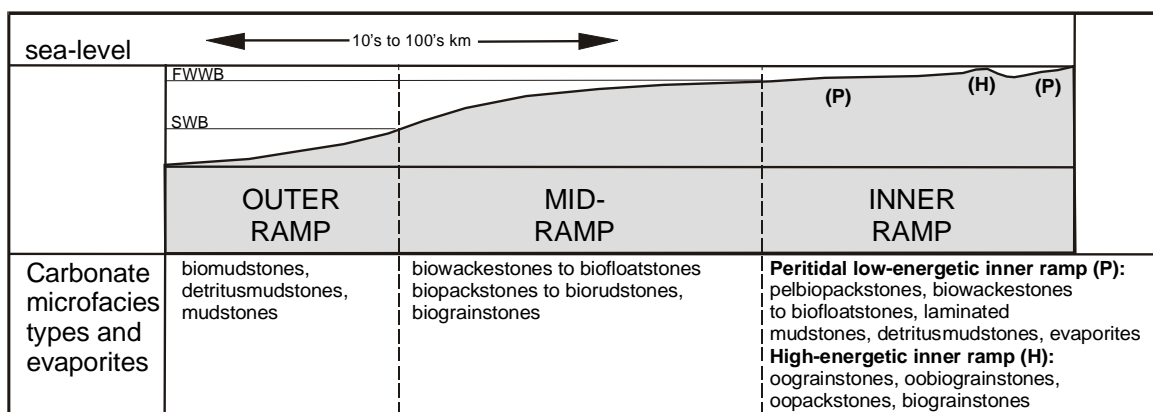
Figure 4-6: The arrangement of carbonate microfacies types and evaporites in inner, middle and outer ramp settings in the "Sundance Basin". FWWB = fairweather wave base, SWB = storm wave base.
