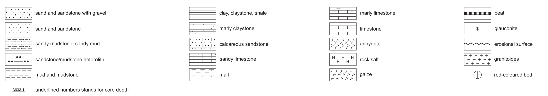
Fig. 3. Lithologic-stratigraphical section of the Malbork IG 1 borehole
