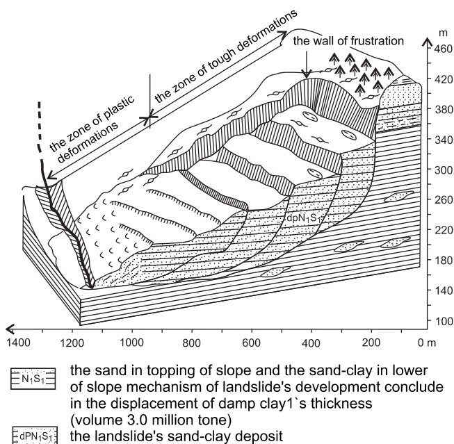
Fig. 4. The principle scheme of the structural-plastic Kostincy landslide (Chernivcy region)
