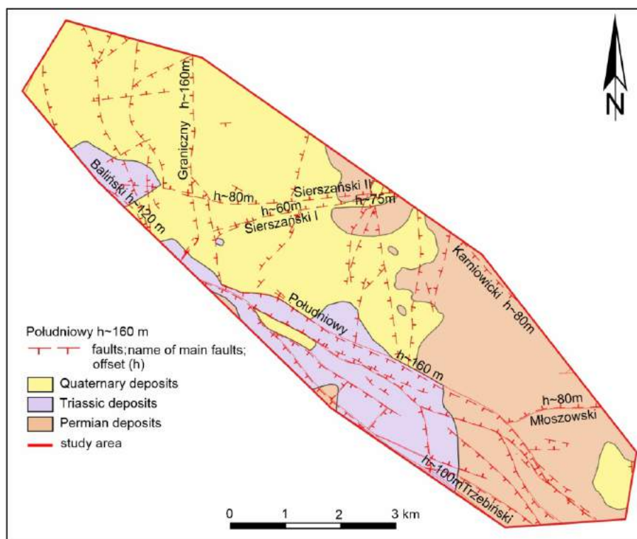
Fig. 3. Carboniferous overburden deposits
